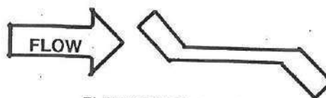
FLOW UNDER SEAT DIAPHRAGM FAILURE = VALVE FAILS TO CLOSE
