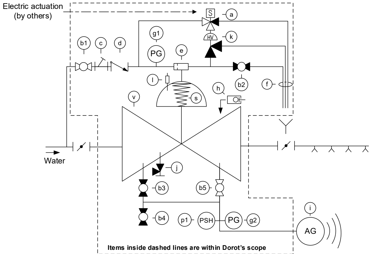
Fig. 2- System P&ID
