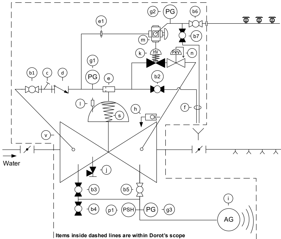
Fig. 2- System P&ID
