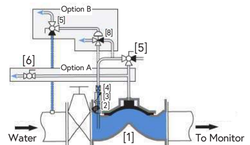
MO\RC Remote Hydraulic Actuation
