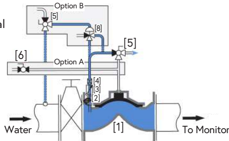
MO\EL Electrical Actuation 6" & larger
