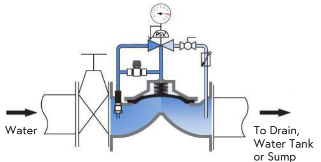
Pressure Relief: 4"- 8"
