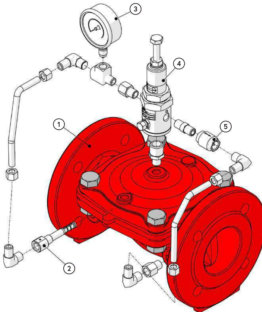
OCV 77 PS\UL: 3"
