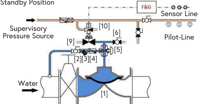
Pneumatically Actuated
