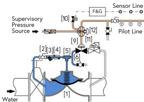
Standby Position
