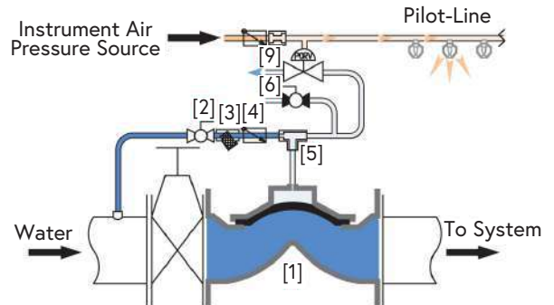
Pneumatically Actuated
